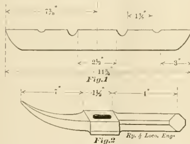
COAL PICK MADE FROM WASTE END OF STEEL BAR.
